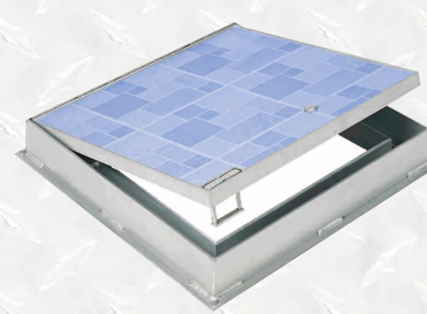
R-TPS Recessed Floor Door 1" [25mm] recess for concrete, stone or architectural tile
